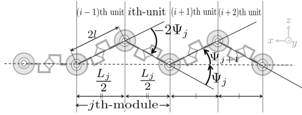
Figure 9. Joint angle for preventing robot slip in vertical pipe.
