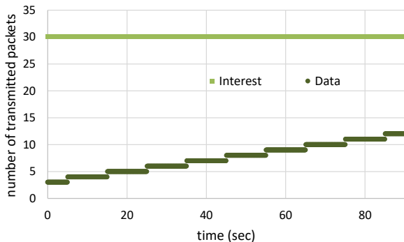
Figure 11. Time variation of transmitted packets for REMIF.
