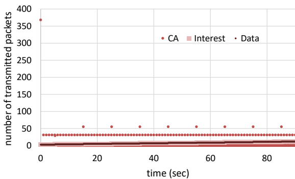
Figure 10. Time variation of transmitted packets for TOP-CCN.
