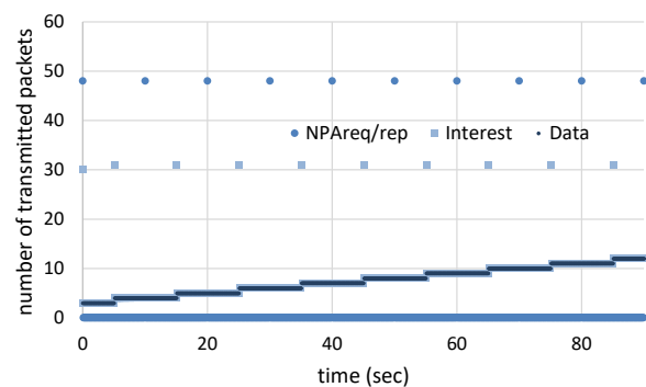
Figure 9. Time variation of transmitted packets for proposal.
