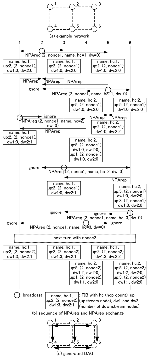
Figure 3. Communication sequence at producer side.
