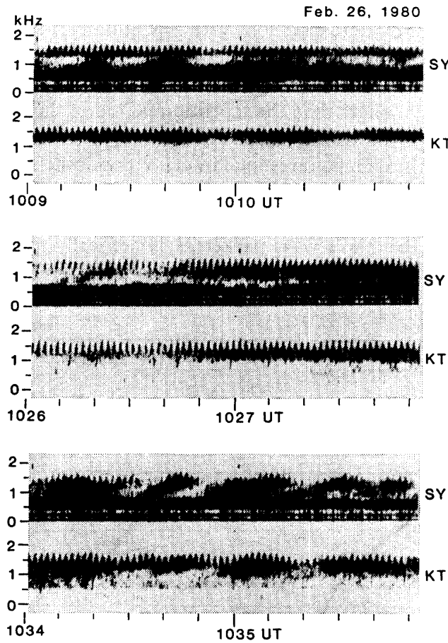
Fig. 2. Frequency-time display of VLF emission observed on February 26, 1980 at Syowa (SY) and at Kitdalen (KT). Rising-tone emissions with repetition period of 20 s are quasi-periodic emissions and a series of discrete emissions with repetition period of 1.7 s are periodic emissions.
