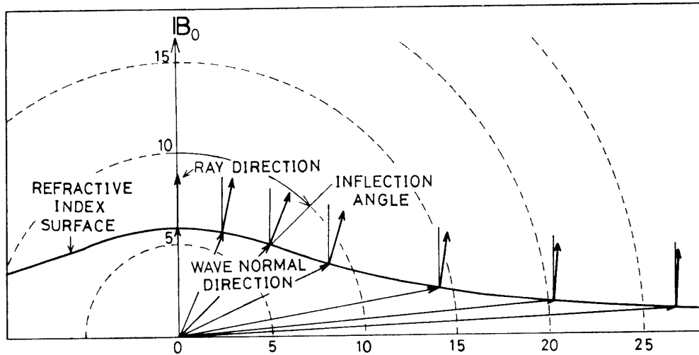
Fig. 17. The relation between the wave normal direction and the ray direction for the refractive index surface at an altitude of 3000 km.
