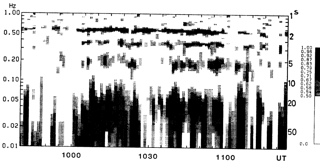
Fig. 10. Time variation of coherency of 1.5 kHz emission intensity between Syowa and Kitdalen.
