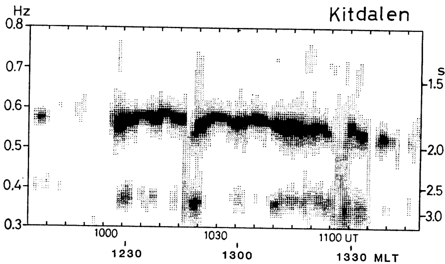
Fig. 9. Same as Fig. 8 except for expanded frequency scale. Gradual increase of the repetition period with magnetic local time, from 1.7 s at 1225 MLT to 1.9 s at 1350 MLT, is recognized.
