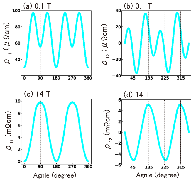
FIG. 4. Angular dependence of \rho_{11} (AMR) and \rho_{12} (PHE) with the current along the binary axis, assuming the mobilities for a thin film.
