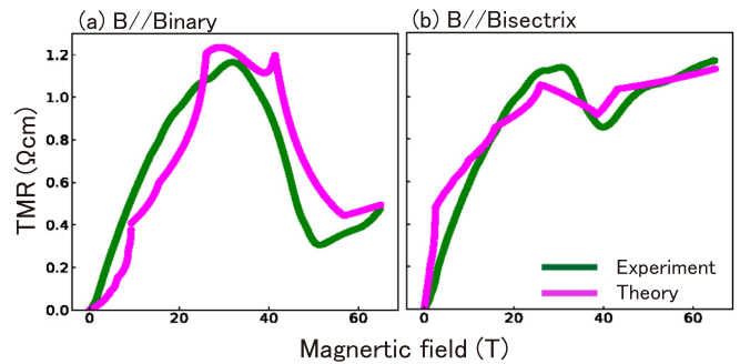
FIG. 5. TMR as a function of magnetic field along the (a) binary axis and (b) bisectrix axis. The theoretical results are obtained by the extended semiclassical theory with the field dependence of mobility. The experimental data are from Ref. [24].
