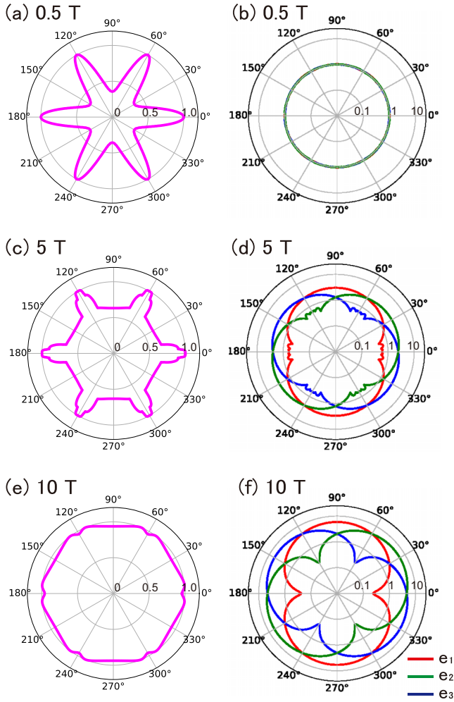
FIG. 2. Left: Angle dependence of inverse TMR with the current along the trigonal axis, \rho_{33}^{-1}(\mathbf{B}) , at 0.5, 5, and 10 T. For easy comparison with the experiment [23], the values of \rho_{33}^{-1} are normalized by its maximum values. Right: Angle dependence of electron carrier densities, n_{e1,e2,e3}(\mathbf{B}) , which are normalized by those in the weak-field limit, n_{ei}(0.1 \text{ T}) = 9.7 \times 10^{16} \text{ cm}^{-3} . 0^\circ and 90^\circ correspond to the binary and bisectrix axes, respectively.
