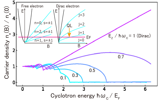
FIG. 3. Magnetic field dependence of carrier density for different Zeeman energies, which characterizes the amplitude of the spin-orbit coupling. The insets show the field dependence of the Landau levels for the free and Dirac electrons.
